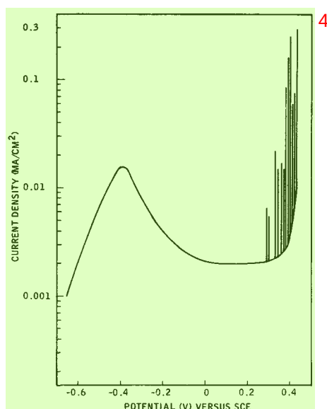
Fig. 5. Anodic polarization curves obtained on a masked electrode for the 17.6% Cr-13.6% Ni-2.93% Mo austenitic stainless steel in argon-saturated 1.0M sodium chloride. The scanning rate was 2000 mv/hr in the positive direction.
